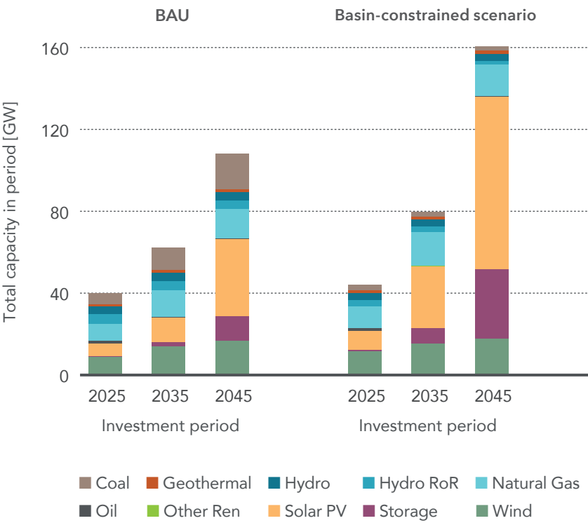
4.3. Installed capacity for reference (BAU) and a scenario that avoided new dams in undeveloped basins (basin-constrained scenario) for Chile by period and technology
