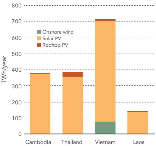
7.7. Low-impact, utility-scale wind and solar energy potential available on converted lands in countries in the Lower Mekong Basin. Modeled technologies include utility-scale wind and PV and rooftop PV.
