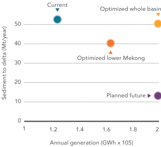
7.8. Various scenarios for hydropower expansion in the Mekong and how they perform in terms of generation and sediment supply.
